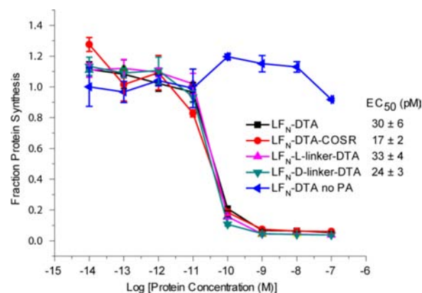
Figure 4. Translocation of LF N -DTA variants into CHO-K1 cells. Cells were incubated with LF N -DTA, LF N -DTA-COSR, LF N -L-linker-DTA, or LF N -D-linker-DTA at different concentrations in the presence or absence of 10 nM PA for 30 min. The media was then replaced with leucine-free media supplemented with 1 μCi/mL 3 H-Leu and incubated for 1 h. After incubation, the cells were washed three times with cold PBS, scintillation fluid was added, and incorporated 3 H-Leu incorporation was determined by scintillation counting. Each data point represents the average of three trials at the specified concentration.
