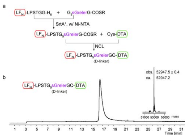
Figure 3. Installing a D-peptide segment between LF N and DTA. (a) Synthetic strategy used to modify the linker region (lower case = D-amino acid). (b) LCMS and deconvoluted MS (inset) for LF N -D-linker-DTA. The reaction conditions are reported in the Supporting Information. LCMS traces are shown as total ion current.
