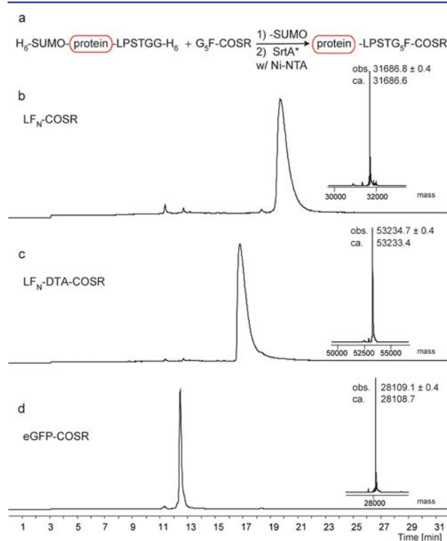
Figure 2. LCMS data for protein \alpha thioester synthesis using SrtA*. (a) SML of model proteins. (b)-(d) LCMS and deconvoluted MS (inset) of the main component for LF N , LF N -DTA, and eGFP thioesters. Reaction conditions: (1) SUMO cleavage: 1 \mu g of SUMO protease per 1 mg of protein for 90 min at room temperature. (2) SML: 500 \mu M G 5 F-COSR, 100 \mu M protein-LPSTGG, 5 \mu M SrtA*, 75 \mu L of Ni-NTA agarose slurry per mg protein, SrtA* buffer, pH 7.0, 30 min. LCMS traces are shown as total ion current.
