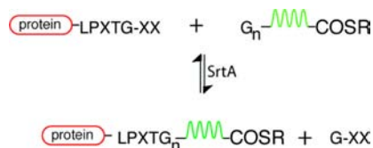
Scheme 1. Protein \alpha Thioester Synthesis Using SrtA
