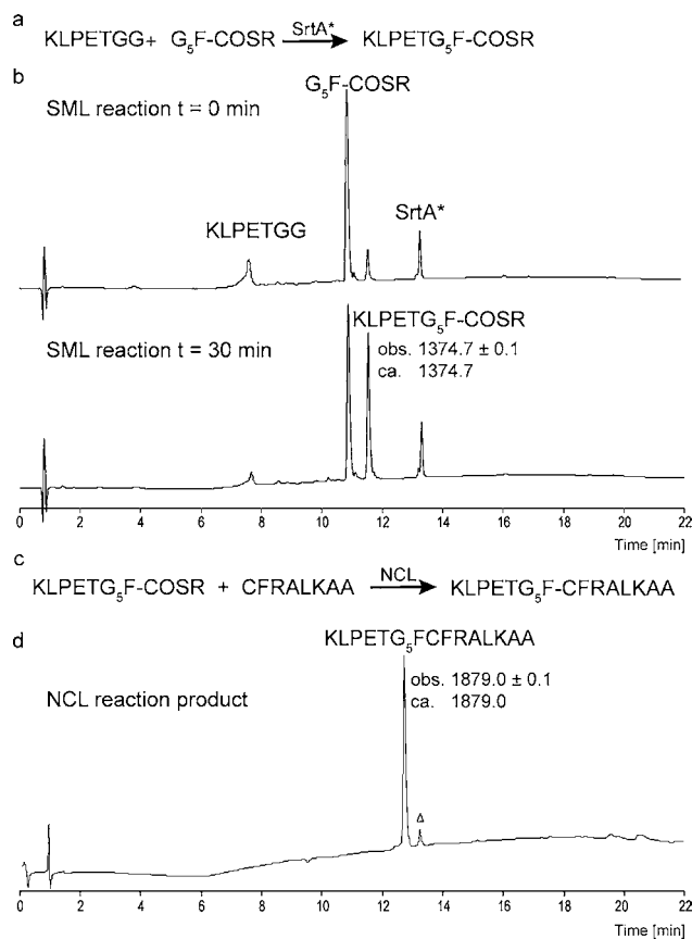
Figure 1. LC data for peptide \alpha thioester synthesis using SrtA* followed by NCL. (a) SrtA*-mediated ligation (SML) of model peptide. (b) Analytical RP-HPLC of crude SML reaction for t = 0 min and t = 30 min. Reaction conditions: 1 mM G 5 F-COSR, 500 \mu M KLPETGG, 5 \mu M SrtA*, SrtA* buffer, (10 mM CaCl 2 , 50 mM Tris, 150 mM NaCl) pH 7.5. (c) Native chemical ligation (NCL) with sortagged thioester reaction product. (d) Analytical RP-HPLC of purified NCL reaction product. Reaction conditions are reported in the Supporting Information. All analytical RP-HPLC signals are measured at 214 nm. The thioester R group was -CH 2 -CH 2 -L-R-CONH 2 . \Delta : impurity peak.
